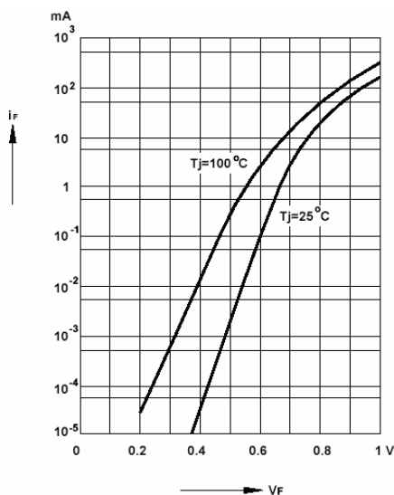
Forward characteristics
